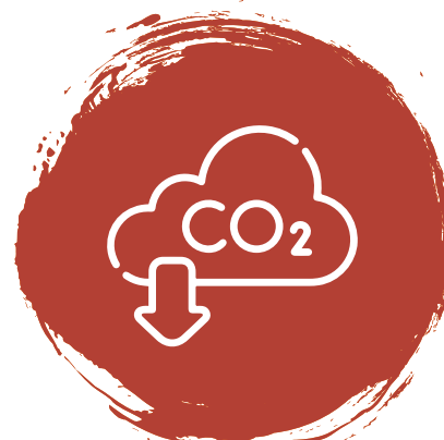
GHG emissions
